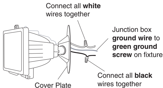
Wiring Fixture
